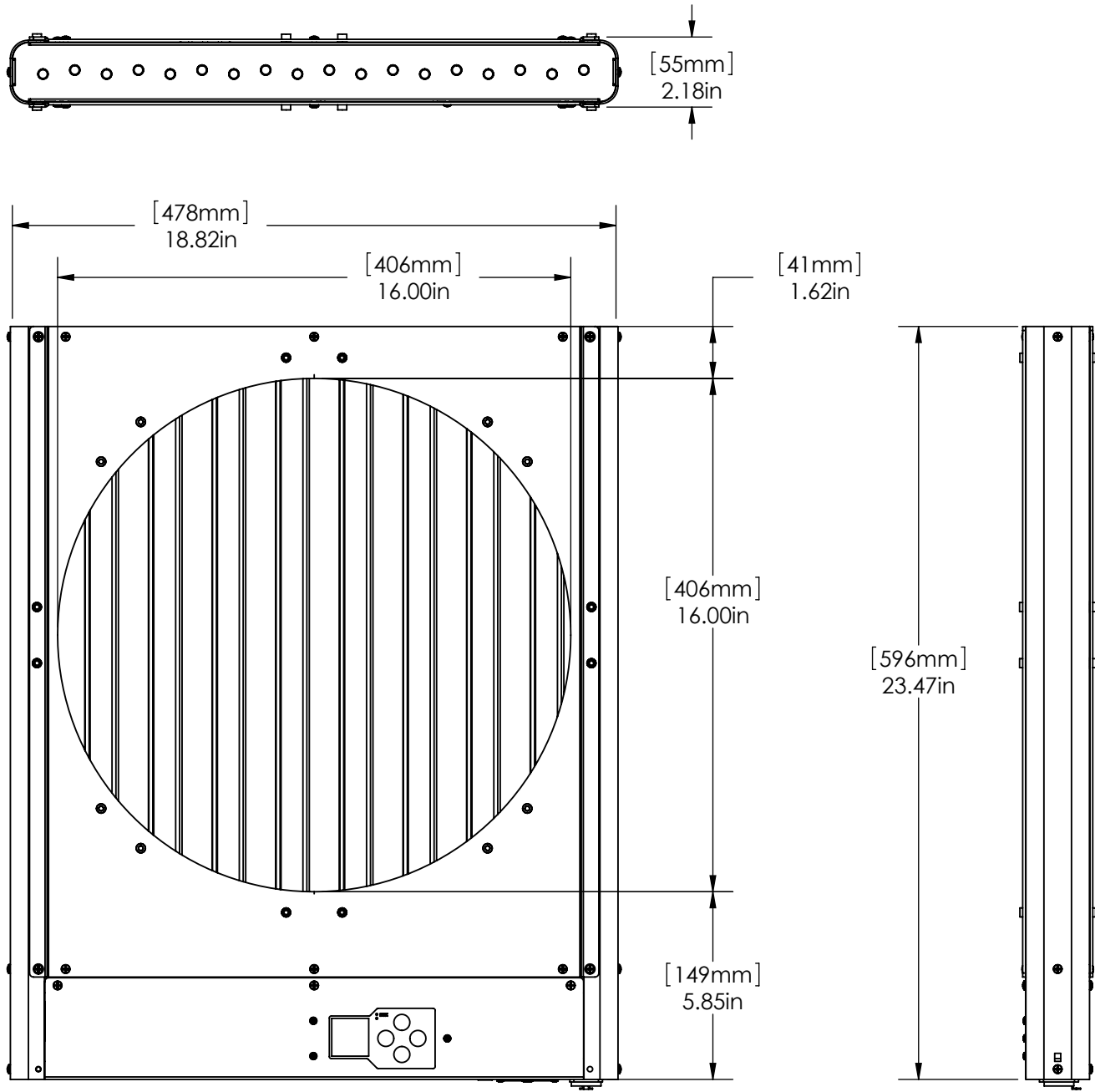
817010 - 5k SHUTTER
